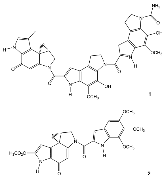
Scheme 1. Structure of (+)-CC-1065 ( 1 ) and (+)-duocarmycin SA ( 2 ).
