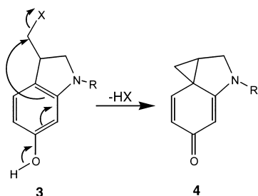
Scheme 2. Formation of the spirocyclopropylcyclohexadienone moiety ( 4 ) from a seco -compound ( 3 ).
