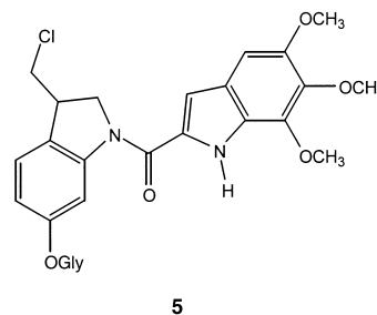
Scheme 3. Prodrugs of the seco -CI-TMI unit ( 5 ).
