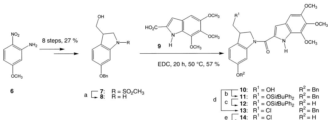
Scheme 4. Synthesis of seco -CI-TMI derivatives 13 and 14 : (a) RedAl, 3 h 110 °C, 94%; (b) t BuPh 2 SiCl, 4-dimethylamino-pyridine, NEt 3 , 16 h 40 °C, 92%; (c) Pd/C, 3 bar H 2 , 16 h, 64%; (d) PPh 3 , CCl 4 , 20 h, 60 °C, 55%; (e) Pd/C, 3 bar H 2 , 24 h, 55%.
