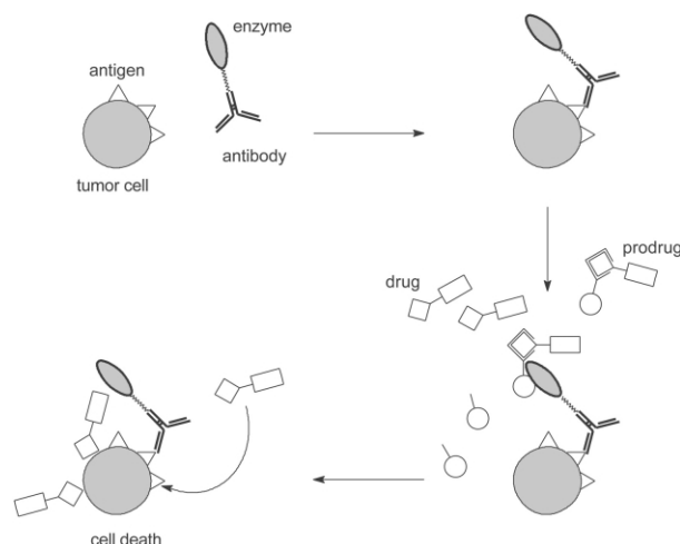
Figure 1. Model of the antibody directed enzyme prodrug therapy (ADEPT) concept.
