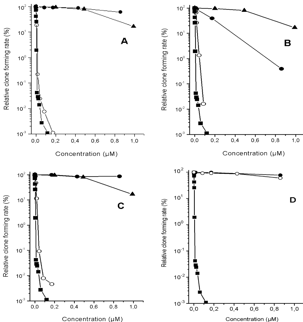
Figure 2. In vitro cytotoxicity of 13 , 14 and 17a–c against human bronchial carcinoma cells of line A549. (A) in vitro cytotoxicity of compound 13 (▲), 14 (■) and 17a without (●) and with (○) addition of \beta -D-galactosidase (0.4 U/mL); (B) in vitro cytotoxicity of compound 13 (▲), 14 (■) and 17b without (●) and with (○) addition of \beta -D-glucosidase (0.4 U/mL); (C) in vitro cytotoxicity of compound 13 (▲), 14 (■) and 17c without (●) and with (○) addition of \alpha -D-mannosidase (0.4 U/mL); (D) in vitro cytotoxicity of compound 17a at pH 6.2 (●) and pH 7.4 (○) and compound 14 (■). Cells were exposed to various concentrations of the test substances for 24 h at 37 °C; after 12 days of incubation clone formation was compared to untreated control assay and the relative clone forming rate was determined.
