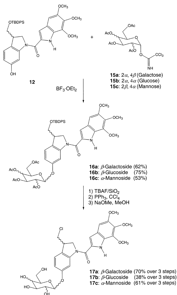
Scheme 5. Synthesis of the glycosidic prodrugs 17a–c of seco -CI-TMI ( 14 ).
